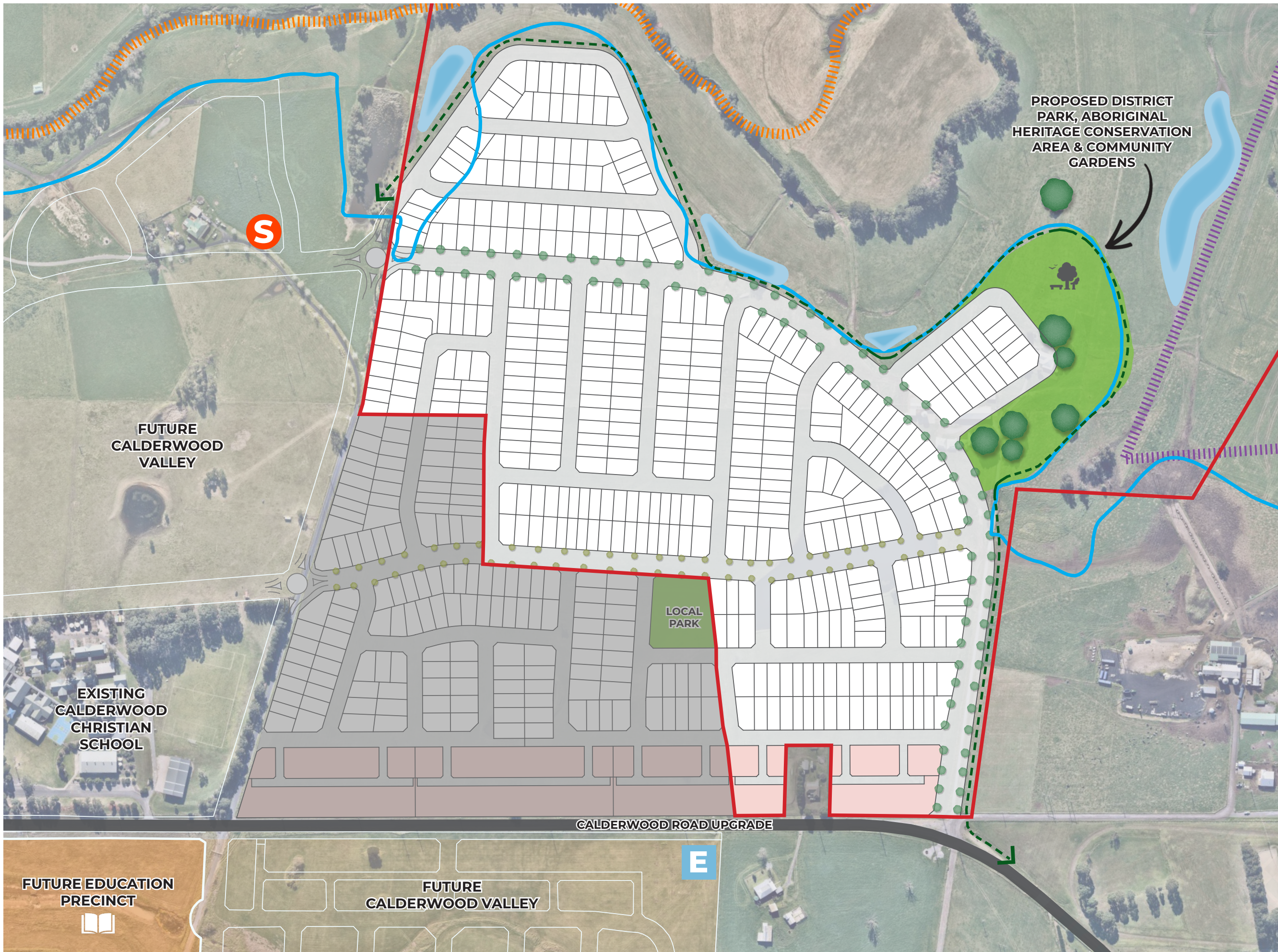
144 CALDERWOOD ROAD, CALDERWOOD CONCEPT LAYOUT PLAN
